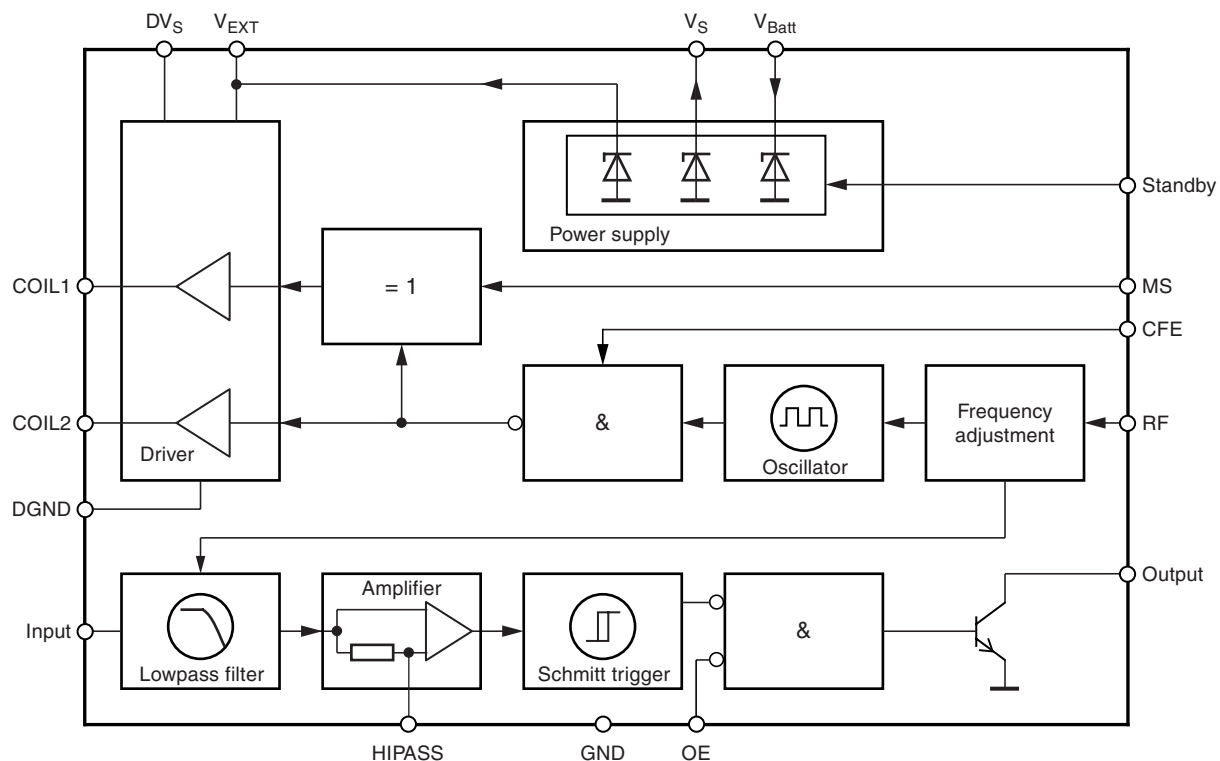
Figure 1-2. Block Diagram
