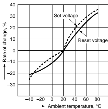
RG2-L2-12V 5 pcs.
