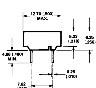
END VIEW
