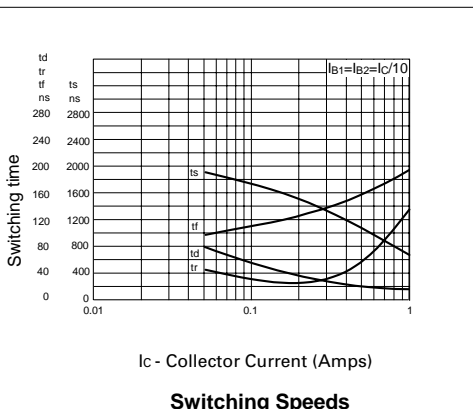
Switching Speeds
