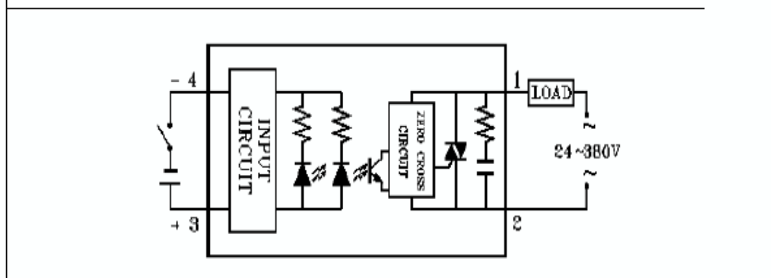
Connection Diagram
