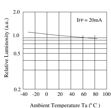
Ambient Temperature vs. Relative Luminosity
