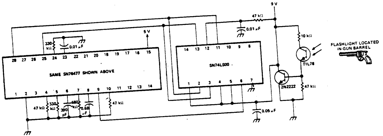
ADDITIONAL CIRCUITRY FOR SILENCER AND GUN SHOT (FOR USE WITH BIRD SOUNDS ABOVE) FIGURE 13
