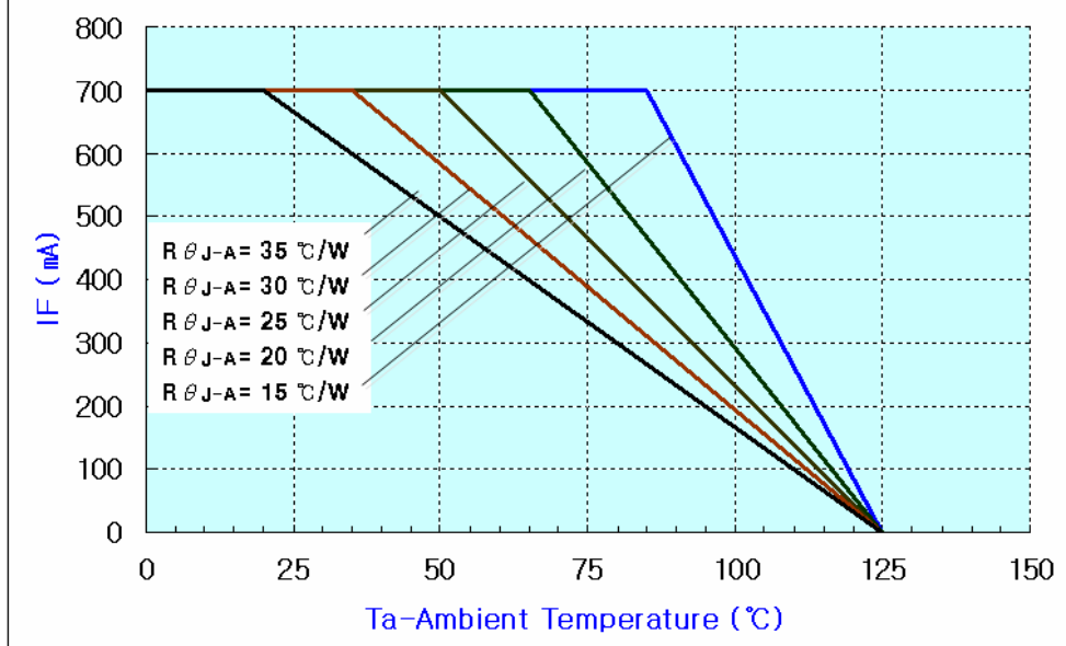
Derating Curve for 700mA (White)
