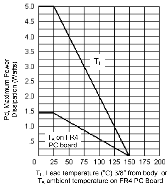
FIGURE 1 Power Derating Curve
