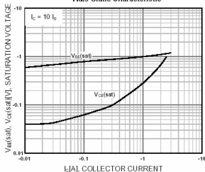
Fig.5 Base-Emitter Saturation Voltage Collector-Emitter Saturation Voltage
