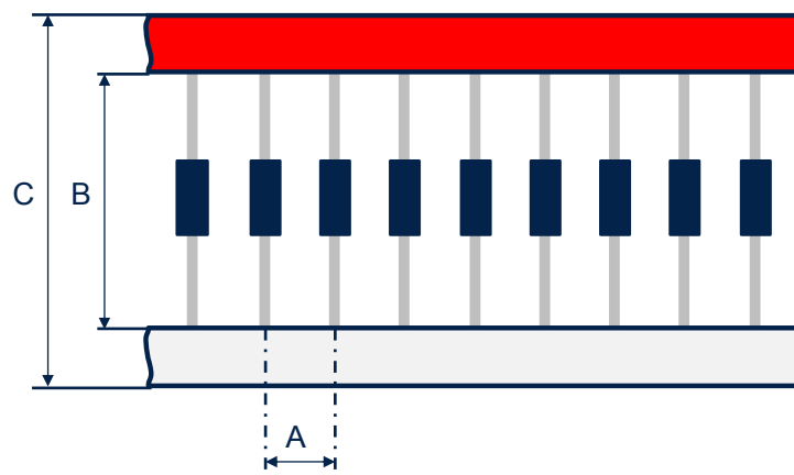
Figure 19. Tape outline
