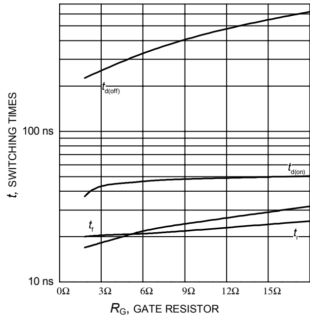
Figure 10. Typical switching times as a function of gate resistor (inductive load, T_J=150^{\circ}\text{C} , V_{CE}=400\text{V} , V_{GE}=0/15\text{V} , I_C=50\text{A} , Dynamic test circuit in Figure E)
