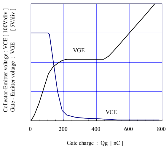
Dynamic Gate charge (typ.) Vcc=300V, Ic=200A, Tj=25°C
