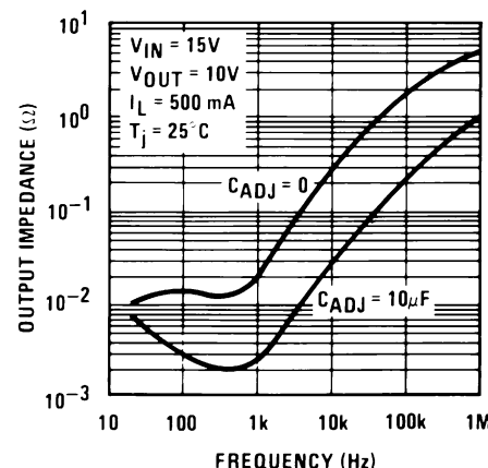
Figure 10. Output Impedance
