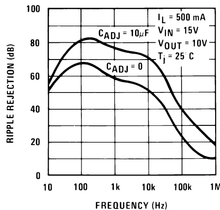
Figure 8. Ripple Rejection
