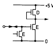
Fig. 7: Pin 10, Input/Output
