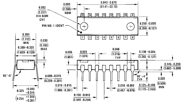
Molded Dual-In-Line Package (N)
