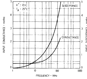
INPUT ADMITTANCE AS A FUNCTION OF FREQUENCY
