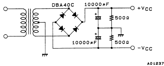
Specified Transformer Power Supply (MG-200 equivalent)
