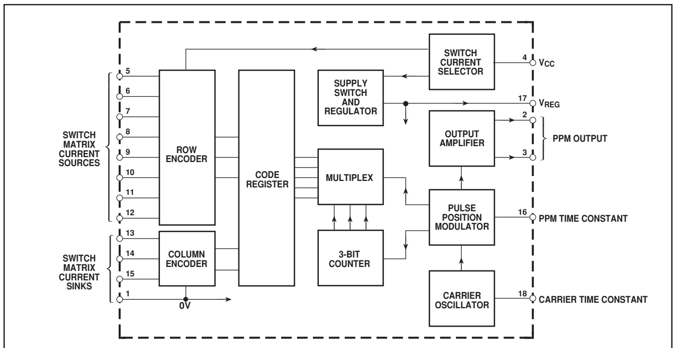
Fig. 2 SL490B block diagram
