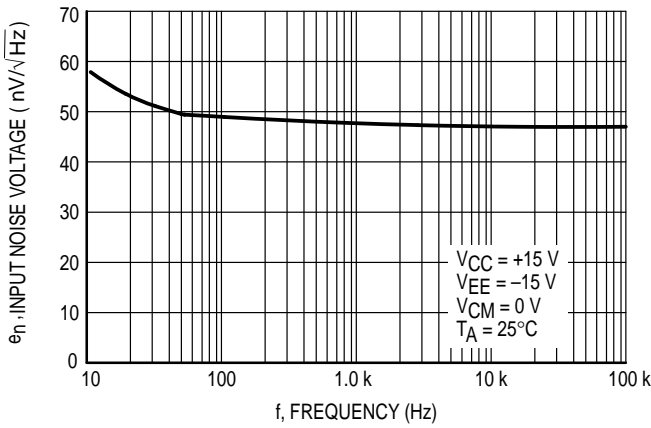
Figure 19. Input Noise Voltage versus Frequency
