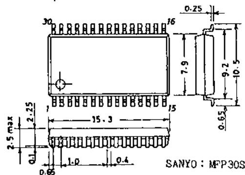
Case Outline 3073A-M30IC [LA7323M] (unit: mm)
