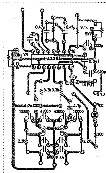
An Example of Printed Pattern Using LC Filter (Cu-foiled area, 50 \times 82 \text{ mm}^2 )
