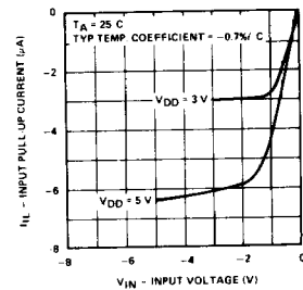
Typical Input Pull-Up Characteristics
