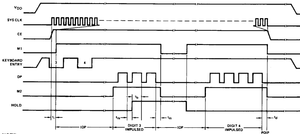
Loop Disconnect Dialler Timing CE-Internal Control Figure 8
