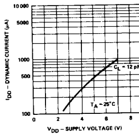
Typical Dynamic Current vs Supply Voltage
