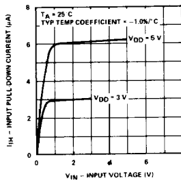
Typical Input Pull-Down Characteristics
