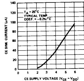
Typical CE Sink Current
