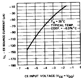
Typical CE Source Current
