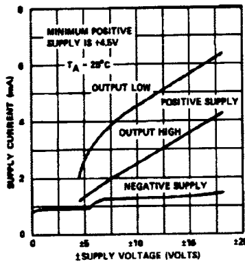
SUPPLY CURRENT vs SUPPLY VOLTAGE
