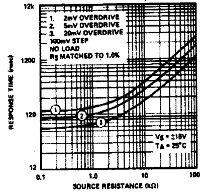
RESPONSE TIME vs SOURCE RESISTANCE
