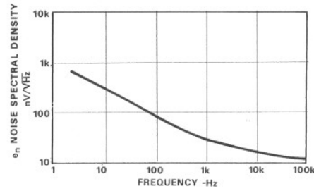
Figure 6. Noise Spectral Density vs. Frequency
