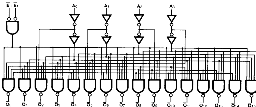
LOGIC DIAGRAM
