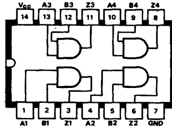
B94 SN74131N Quad 2-input AND power driver (15V)
