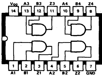
B93 SN74130N Quad 2-input AND power driver (30V)
