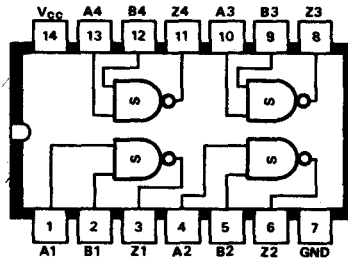
B95 SN74135N Quad 2-input NAND Schmitt
