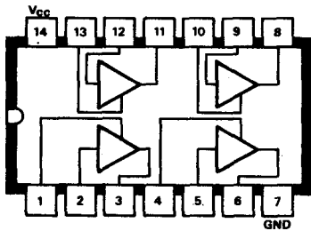
B92 SN74126N Quad Bus Driver
