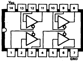
B91 SN74125N Quad Bus Driver
