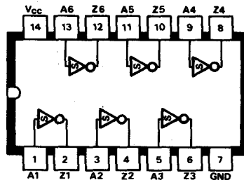
B96 SN74137N Hex Inverter Schmitt
