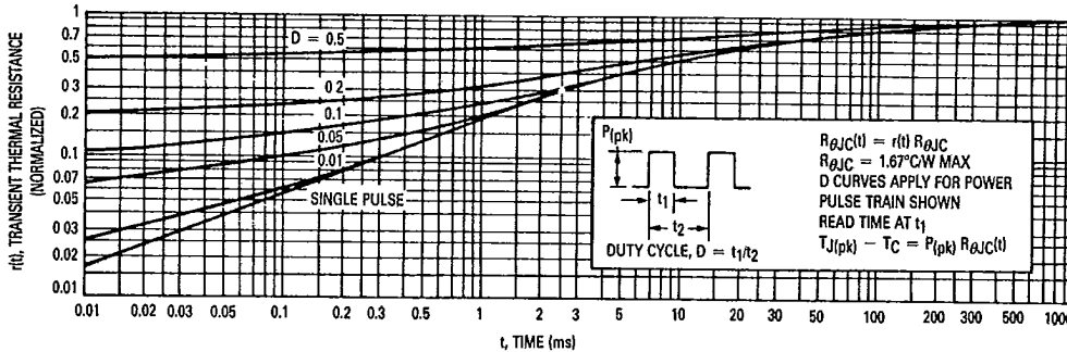
Figure 10. Thermal Response
