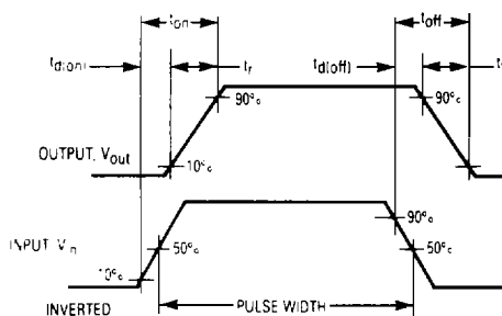
Figure 14. Switching Waveforms
